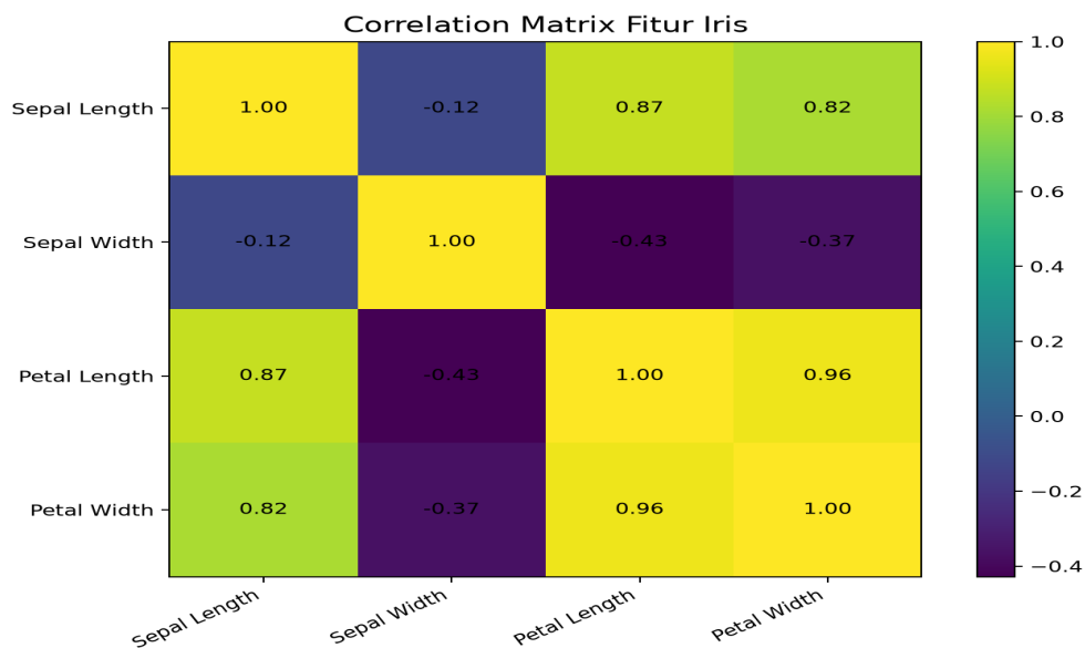
Chart: Correlation Heatmap
